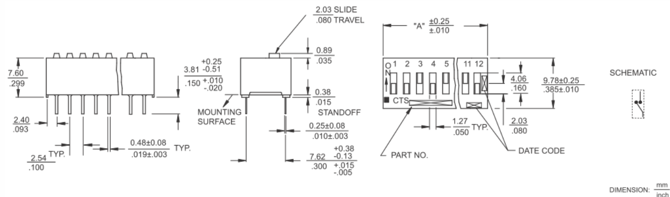
Figure 1 - SPST
